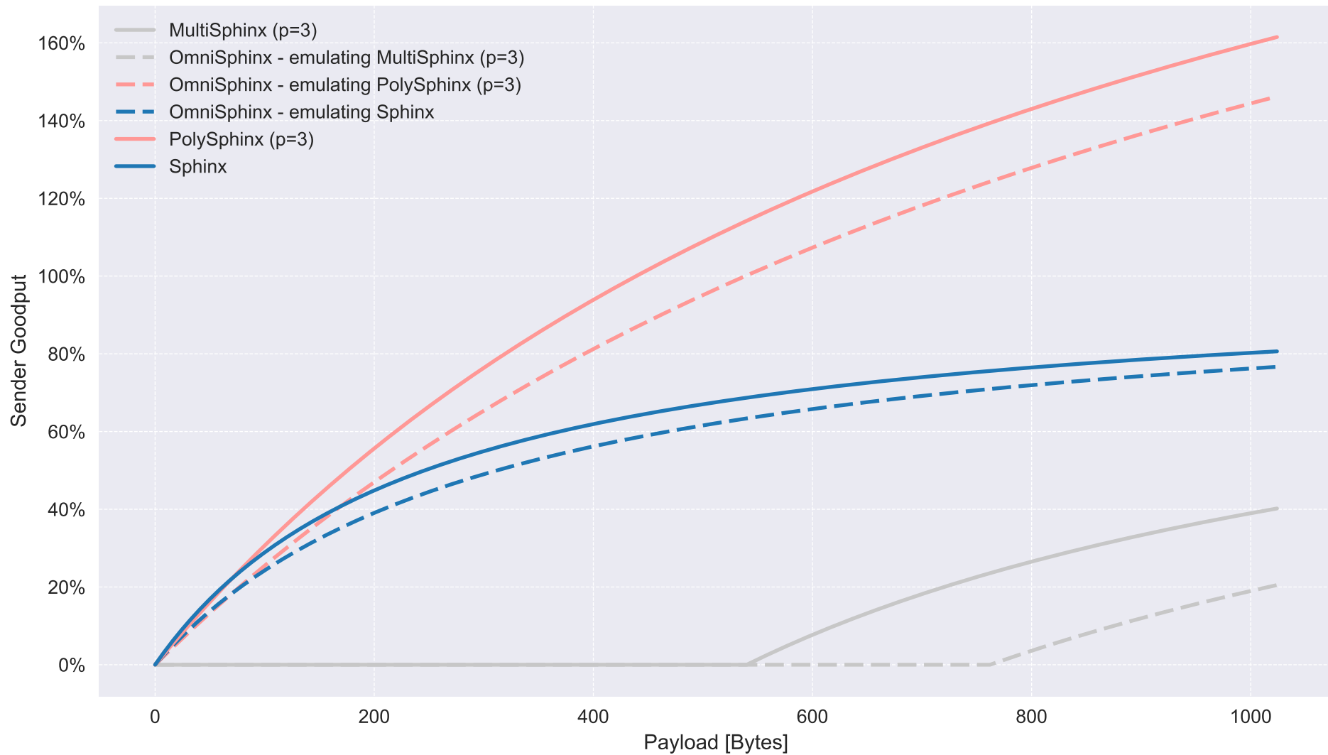
Sender Goodput for OmniSphinx multicast variants with minimal \beta
